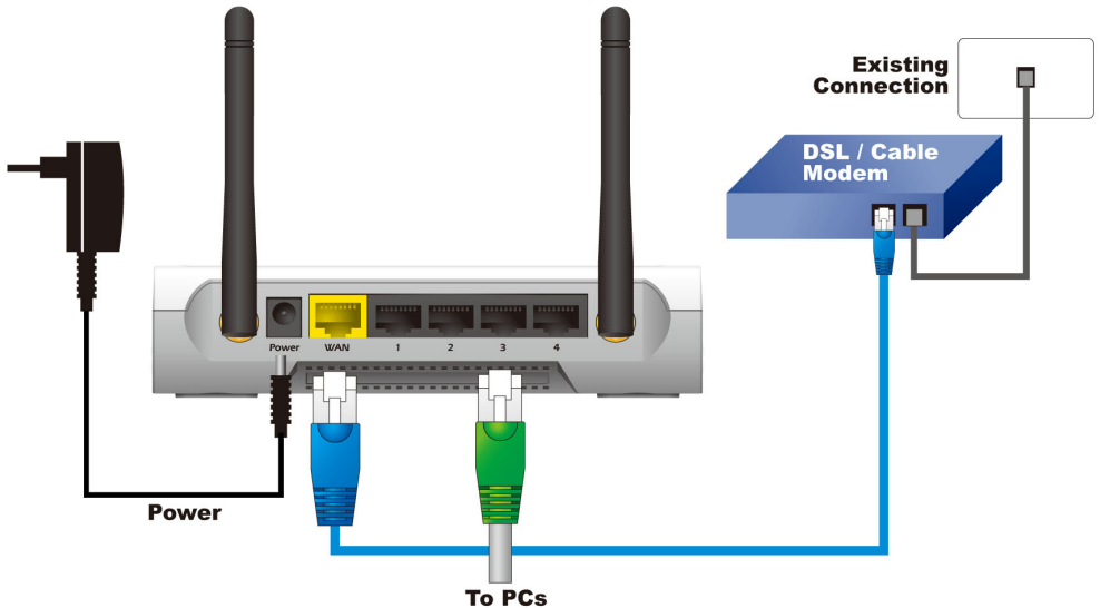
Figure 4: Installation Diagram
