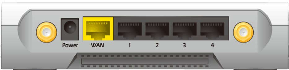
Figure 3: Rear Panel
